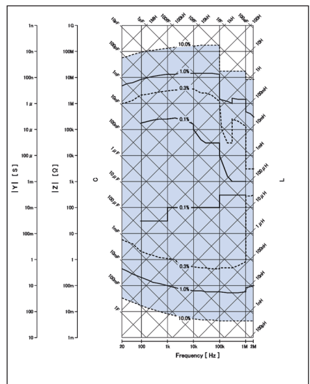
Figure 1. 10% impedance measurement accuracy range. Test signal 1 Vrms, MED mode, cable 0m.
